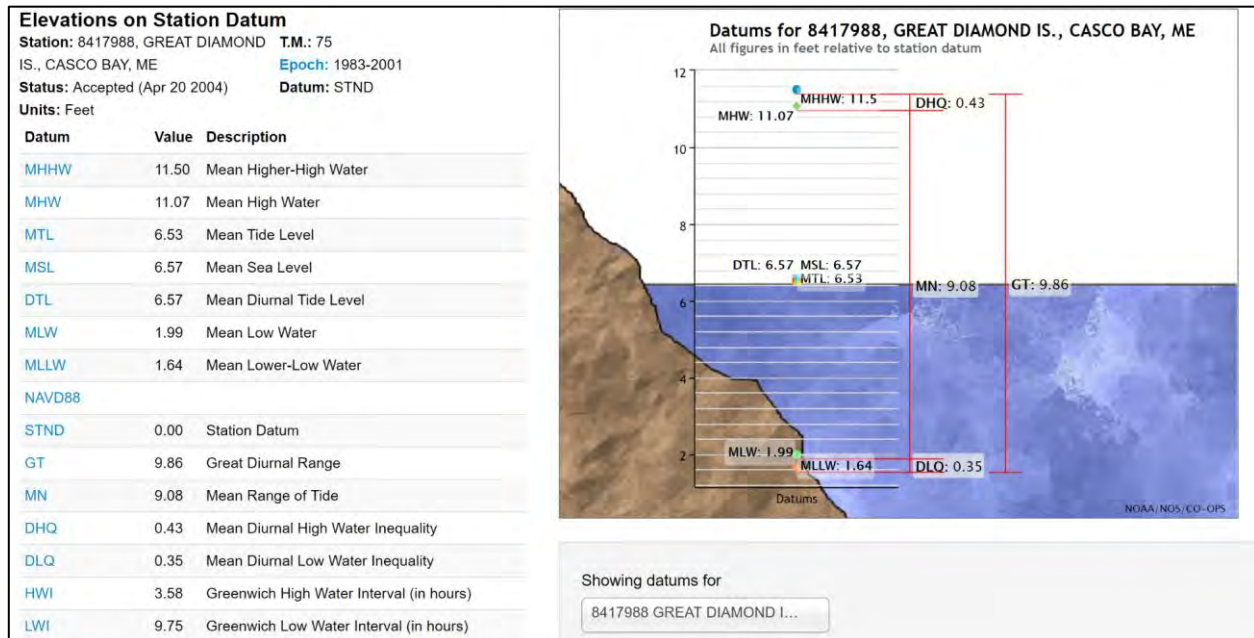
Figure 1: Source: National Oceanographic and Atmospheric Administration (NOAA) Tides & Currents Datum. Note that elevations are given in Station Datum. In this example subtract 1.64 feet, the elevation of MLLW to get values commonly used in tide tables. ( https://tidesandcurrents.noaa.gov/datums.html?id=8417988 )
